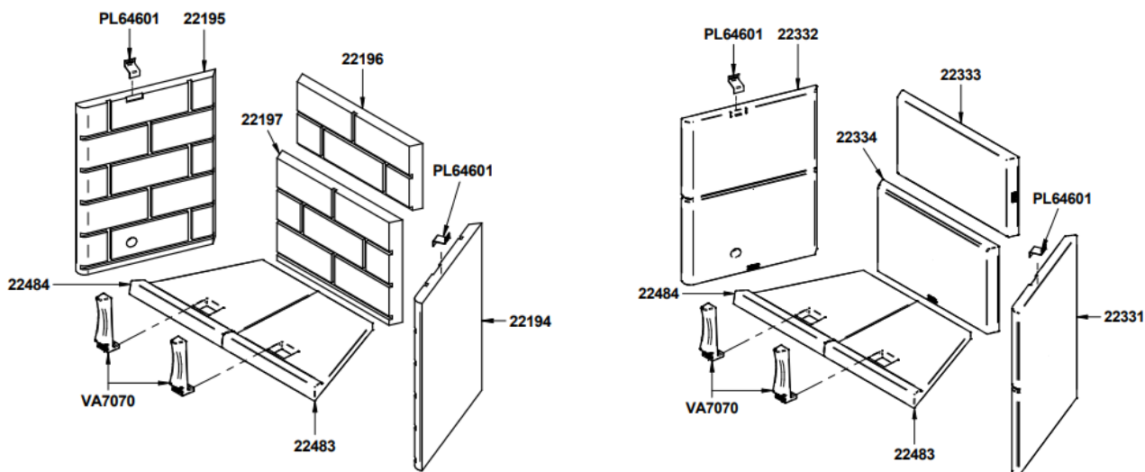
Figure 41: Replacing Antoinette refractory panels
